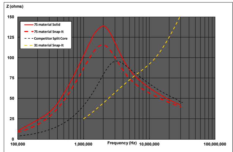
Comparison of Material Cable Cores
