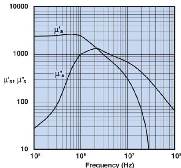
Figure 6 Complex Permeability vs. Frequency Measured on a 2673000301 bead using the HP 4284A and the HP 4291A.
