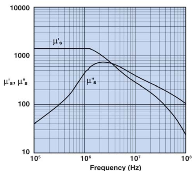
Figure 7 Complex Permeability vs. Frequency Measured on a 17/10/6mm toroid using the HP 4284A and the HP 4291A.
