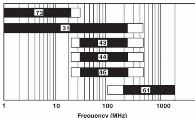
Figure 26 Available Fair-Rite Suppression Materials vs. Frequency
