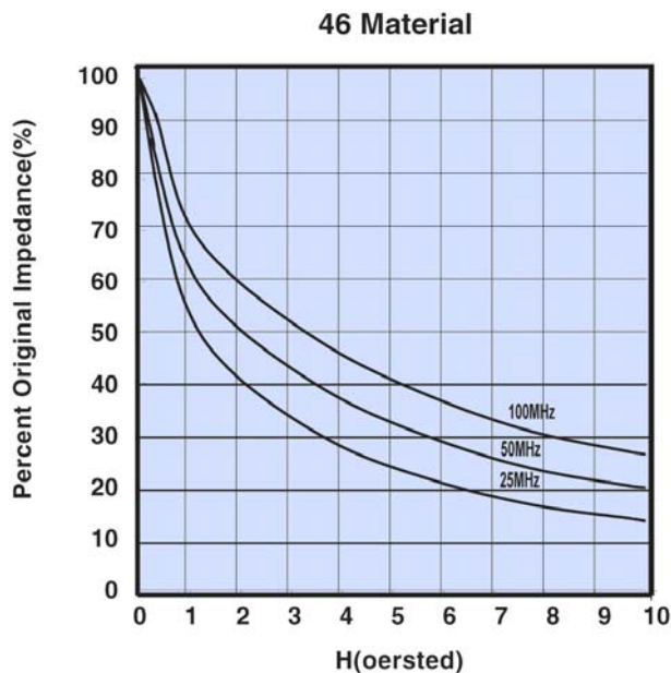
Figure 22 Percent of Original Impedance vs. Magnetic Field Strength. Measured on a 2646000301 using the HP4291A.
