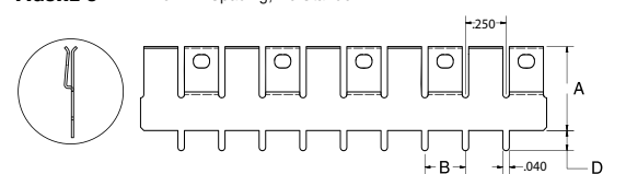
FIGURE 6 .25" Pin Spacing, No Standoff
