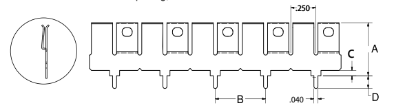
FIGURE 4 1.0" Pin Spacing, No Standoff
