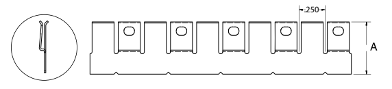
FIGURE 2 .50" Pin Spacing, No Standoff
