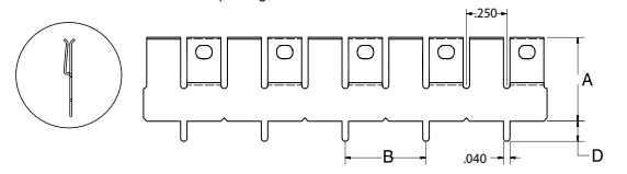
FIGURE 3 .50" Pin Spacing, With Standoff
