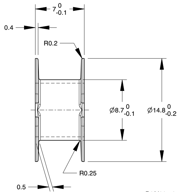
P18/11 - 1 SECTION BOBBIN PART No. P18111
